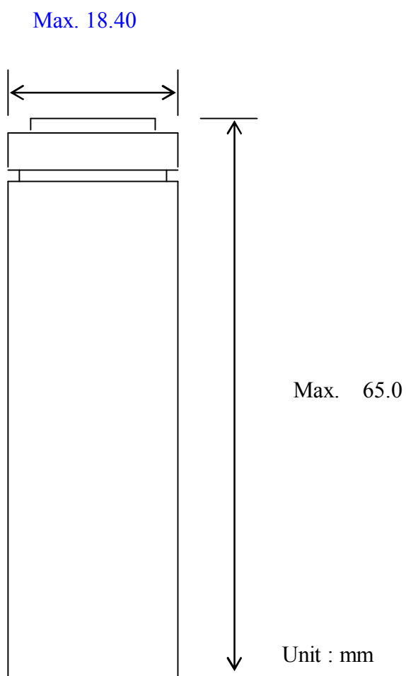
Fig.1. Outline Dimensions of ICR18650-26F
